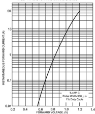
FIG.2 - TYPICAL FORWARD CHARACTERISTICS
